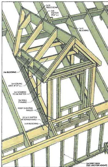
3 DORMER FRAMING PERSPECTIVE SCALE : NA
