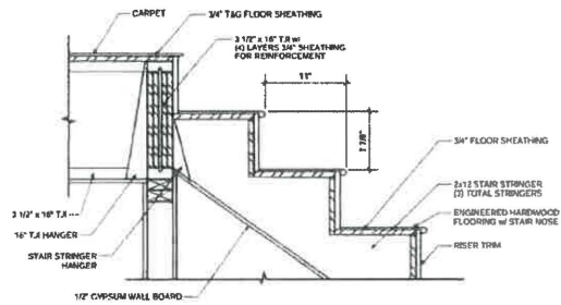
1 STAIR DETAIL SCALE : 1/16" = 1'-0"
