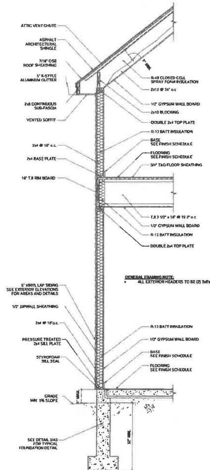
5 WALL SECTION DETAIL SCALE: 3/8" = 1'-0"
