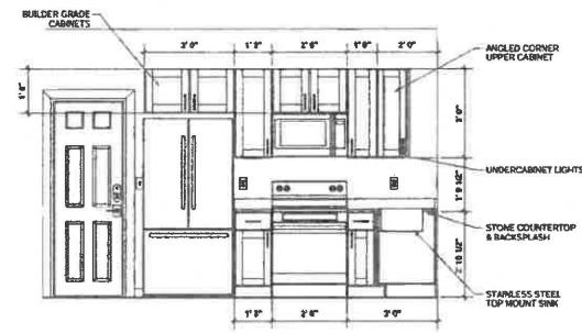
2 KITCHEN ELEVATION SCALE: 1/8" = 1'-0"
