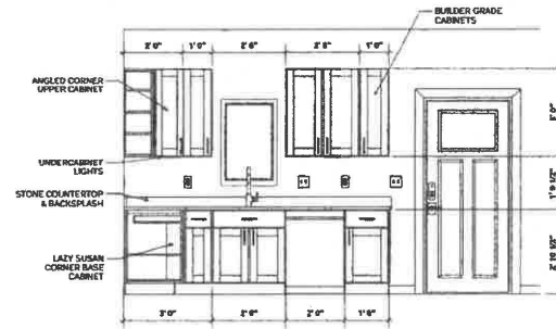
1 KITCHEN ELEVATION SCALE: 1/8" = 1'-0"
