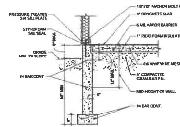
3 TYP. FOOTING DETAIL SCALE: 3/8" = 1'-0"
