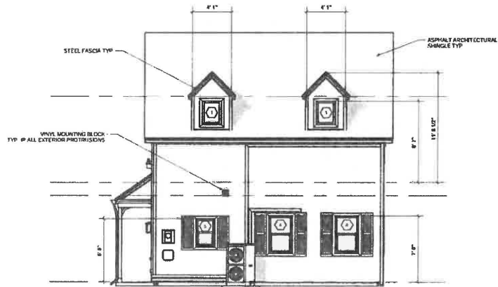
3 WEST ELEVATION - BACK SCALE : 1/8" = 1'-0"
