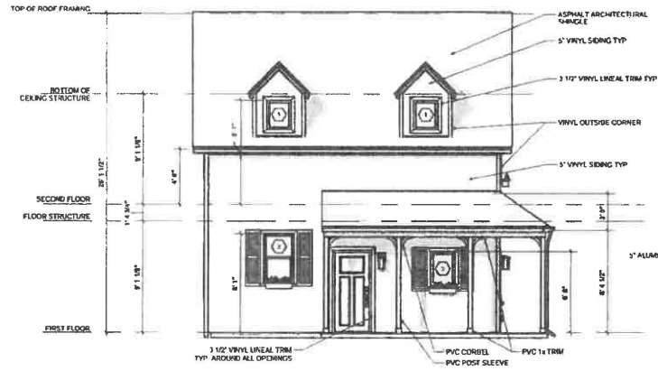
1 EAST ELEVATION - FRONT SCALE : 1/8" = 1'-0"
